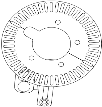
CENTER OF SENSOR NEEDS TO BE CENTERED IN TONE WHEEL "WINDOWS"
