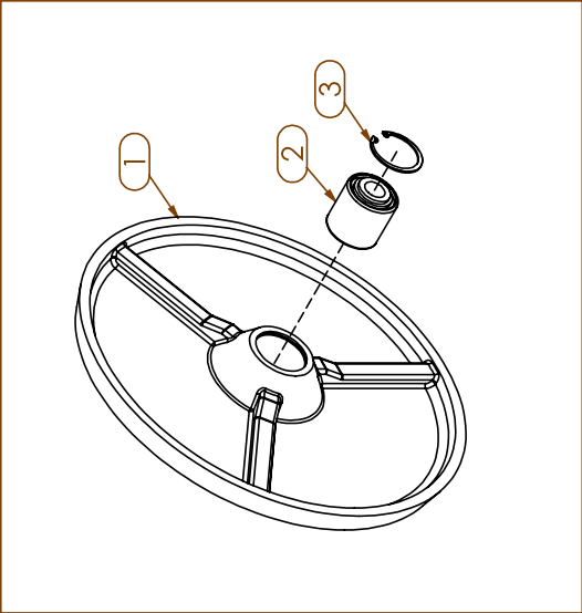
100376 CAST CLOSING WHEEL
