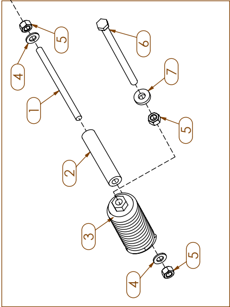
DOWN PRESSURE SPRING (BLACK) ASSEMBLY
