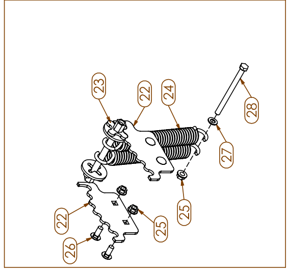
QUICK-ADJUST HD SPRING DOWNFORCE
