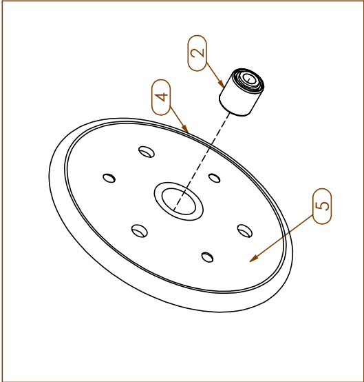
7074.N CLOSING WHEEL
