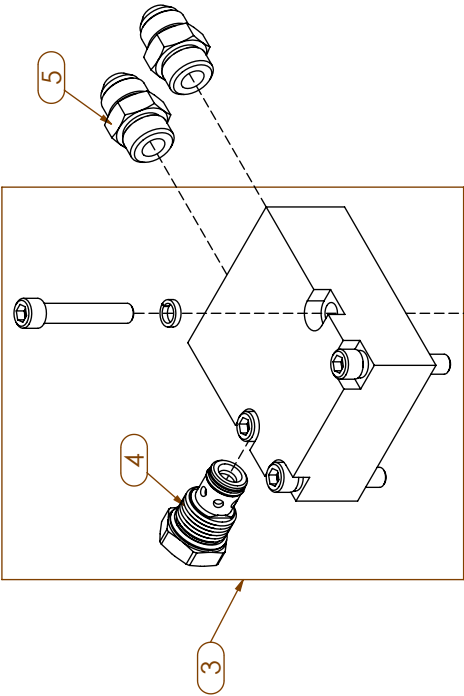
STANDARD TURBOFAN HYDRAULIC MOTOR 2.8 CUBIC INCH DISPLACEMENT
