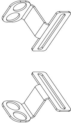
804749 CAN BE MOUNTED IN THE LEFT HAND AND RIGHT HAND ORIENTATION ON THE WHEELBLOCKS
